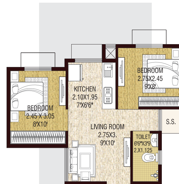
UNIT TYPE - 2BHK WING-E9
