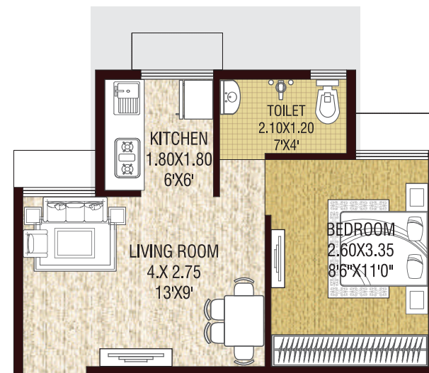
UNIT TYPE - 1BHK WING-E9
